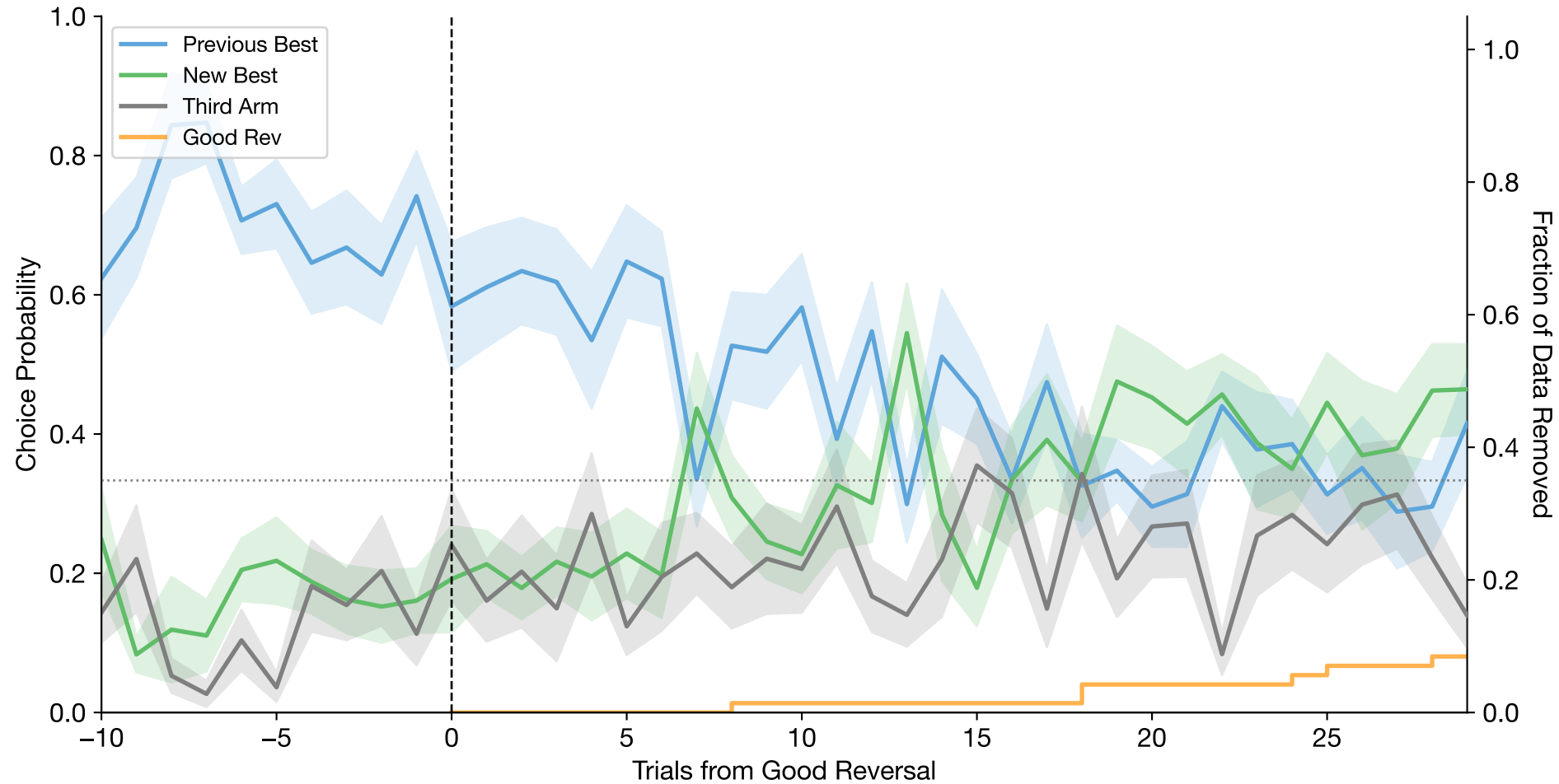
Good Reversal-Aligned Choices (mean \pm se across subjects | n=13 subjects, n=71 reversals)
